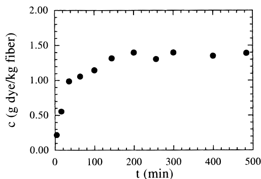
Figure 4. Plot of dye concentration in the fiber as a function of the time of dyeing. The nylon 66 fiber was dyed with fluorescein in an infinite dyebath at pH 6, 95 °C, and the dye concentration in the dyebath was 0.1 g/L.
